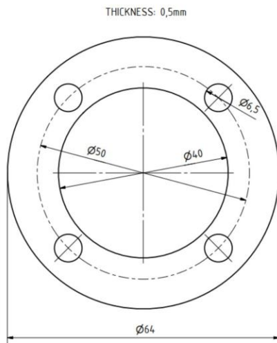
Cylinder Cover
