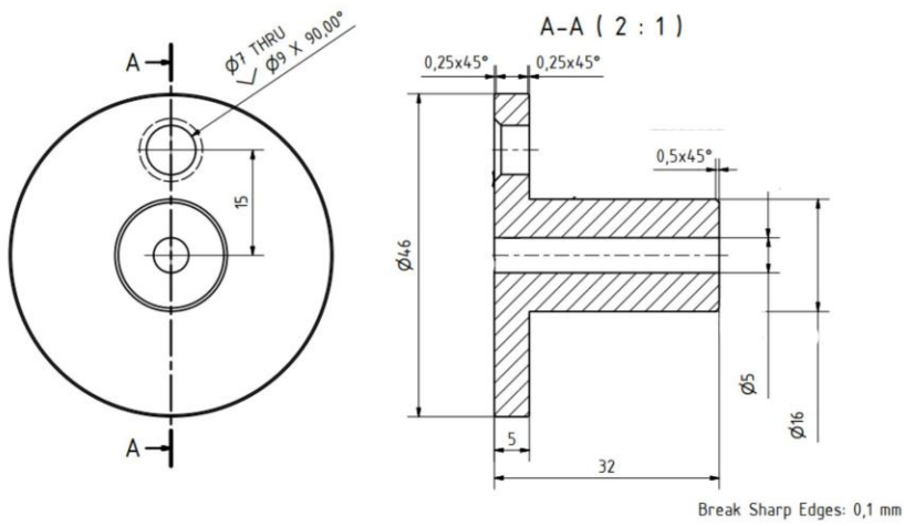
Cylinder Cover
