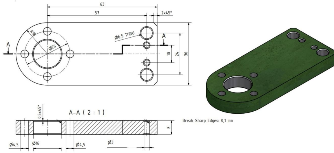
Support
