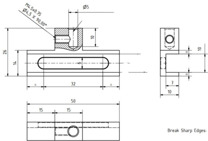
Cross Head
