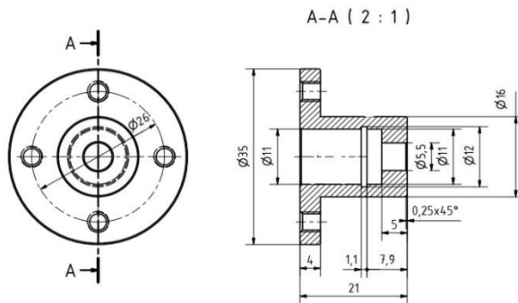
Bearing Support
