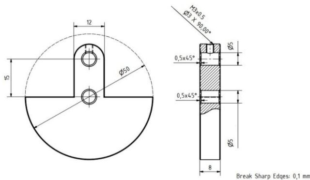
Counter weight A
