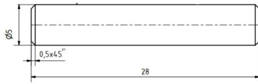
Piston pin
